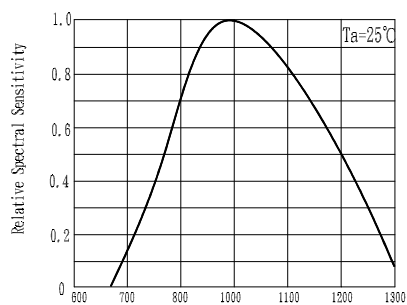
Fig.5 Spectral Sensitivity
