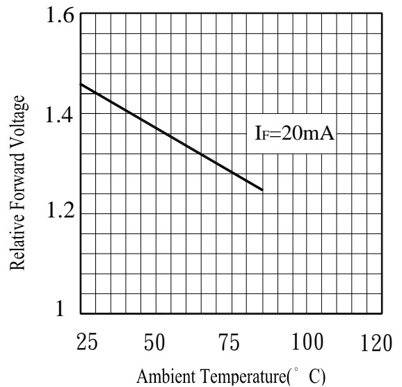
Fig.8 Relative Forward Voltage vs. Ambient Temperature(°C)
